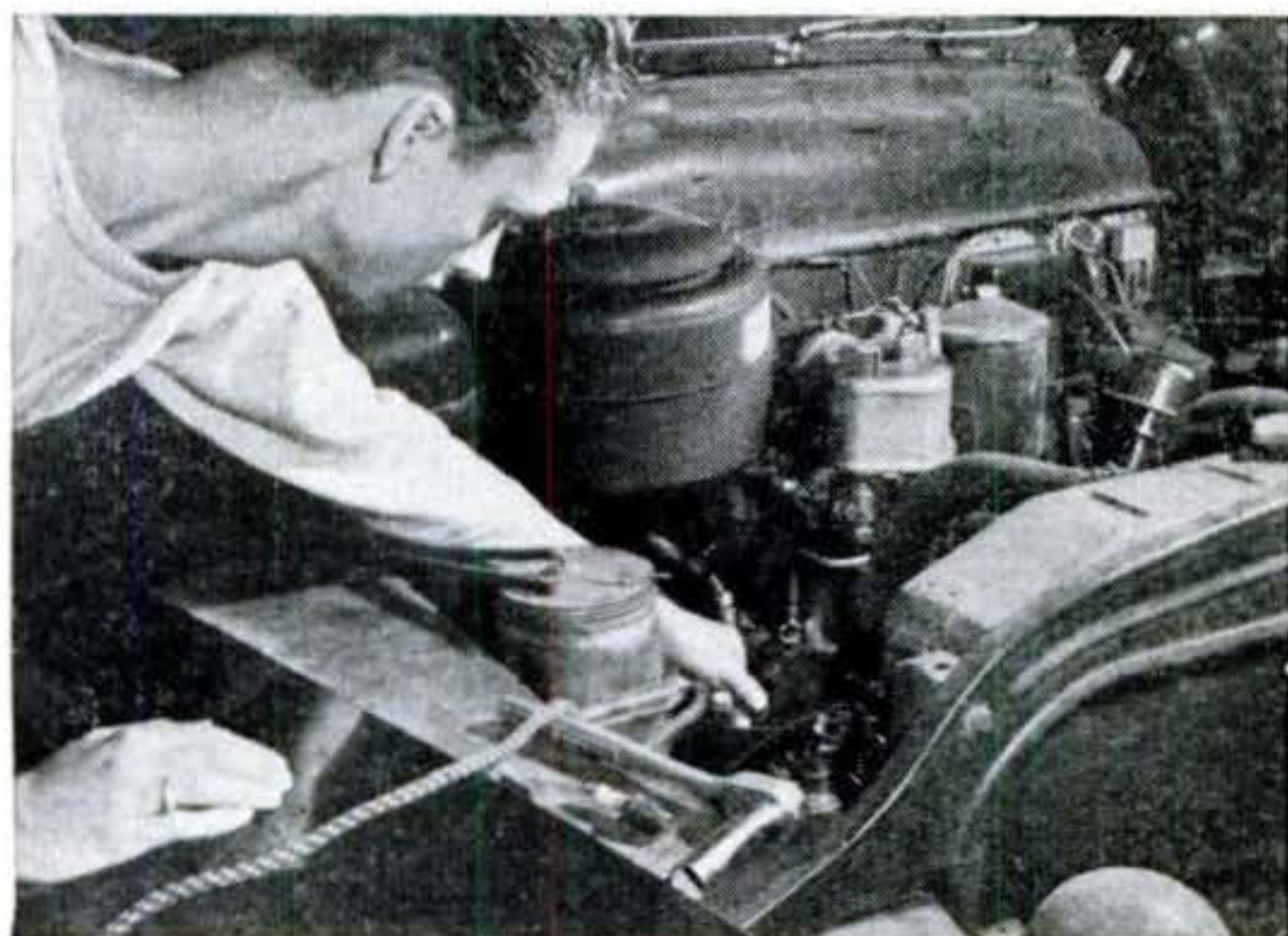
AN OLD SPARK PLUG , converted to an air fitting, is a big help in checking for compression leaks in your auto engine.
